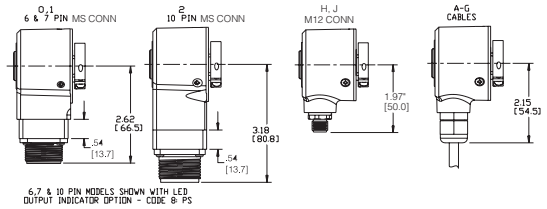
6, 7 & 10 PIN MODELS SHOWN WITH LED OUTPUT INDICATOR OPTION - CODE 8 PS
